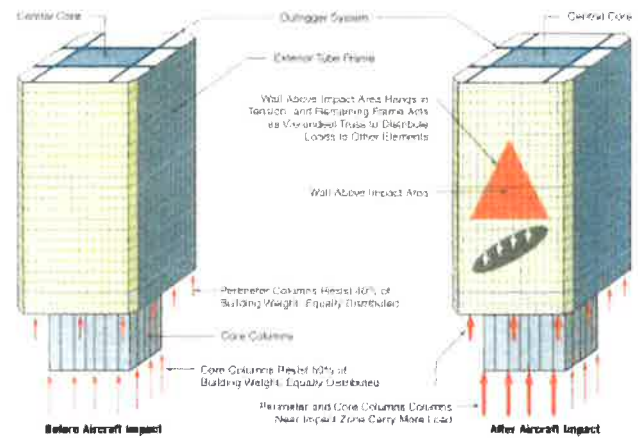
Figure 2. Post-Impact Load Redistribution © NIST
