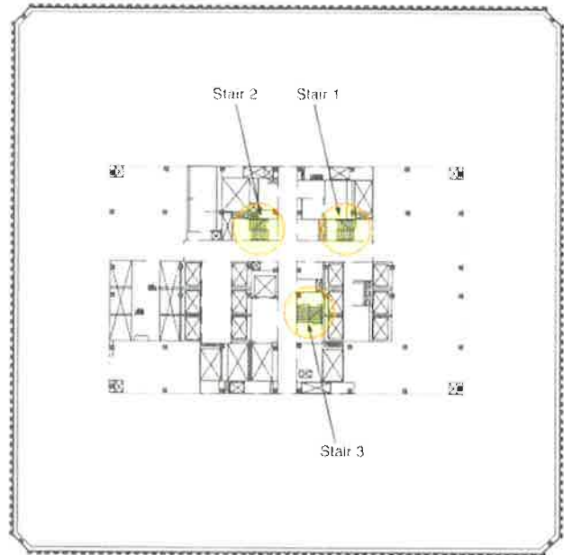
Figure 4. WTC Core Elevator and Stair Layout
