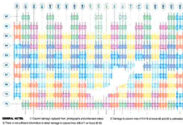
Figure 1. Damage to South Face of WTC 2 © NIST
